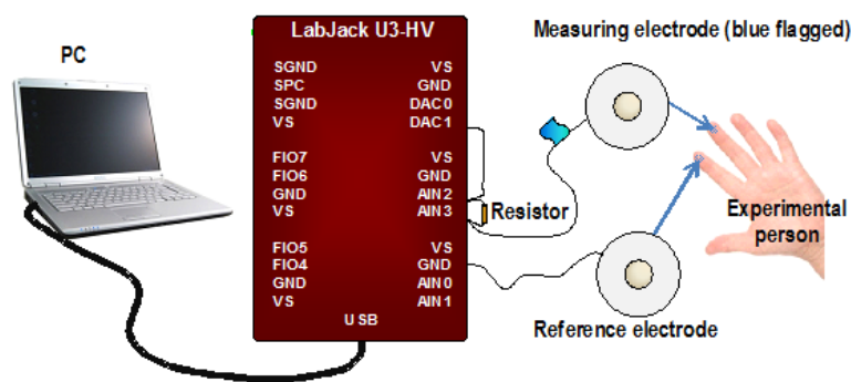
Figure 8.2: Placing of electrodes
