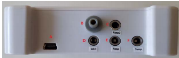
Figure 8.1: Polygraph Bio - connectors
