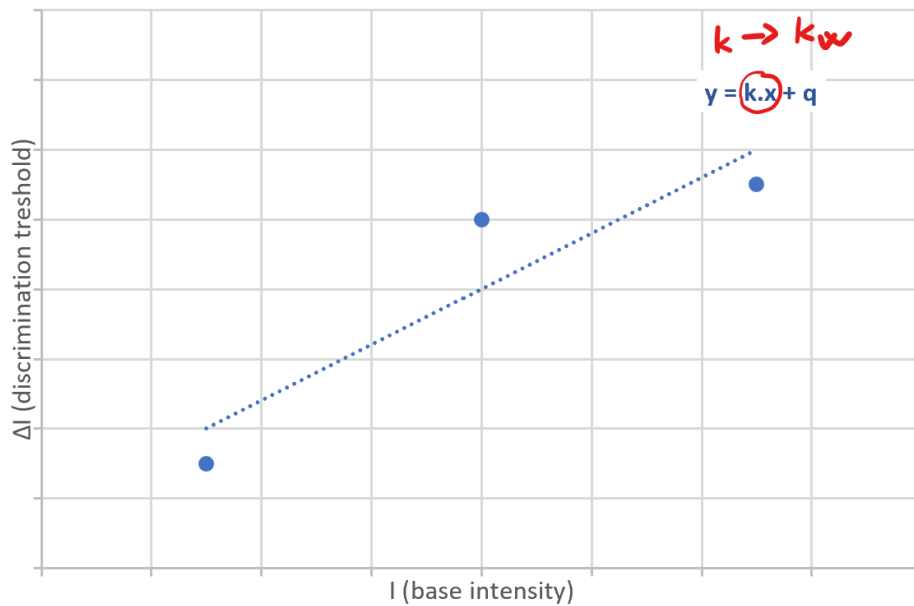
Figure 7.1: Weber fraction
