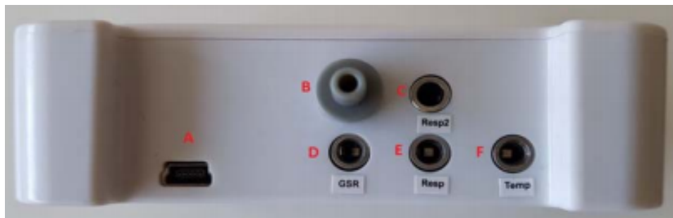
Figure 8.1: Polygraph Bio - connectors
