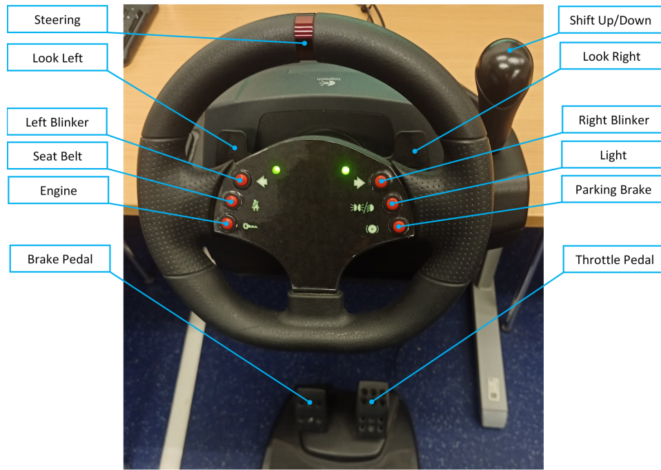
Figure 9.1: Car simulator controls
