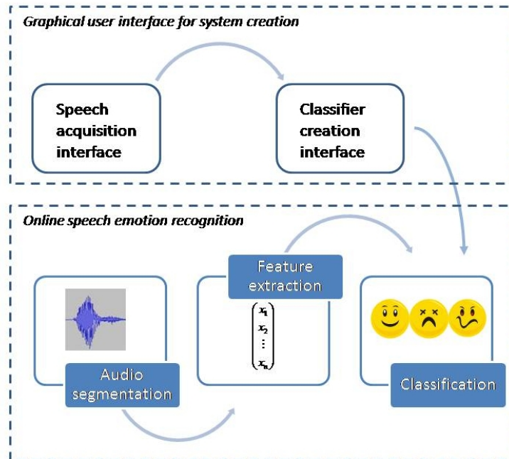
Figure 13.7: Architecture of EmoVoice : 3 steps
